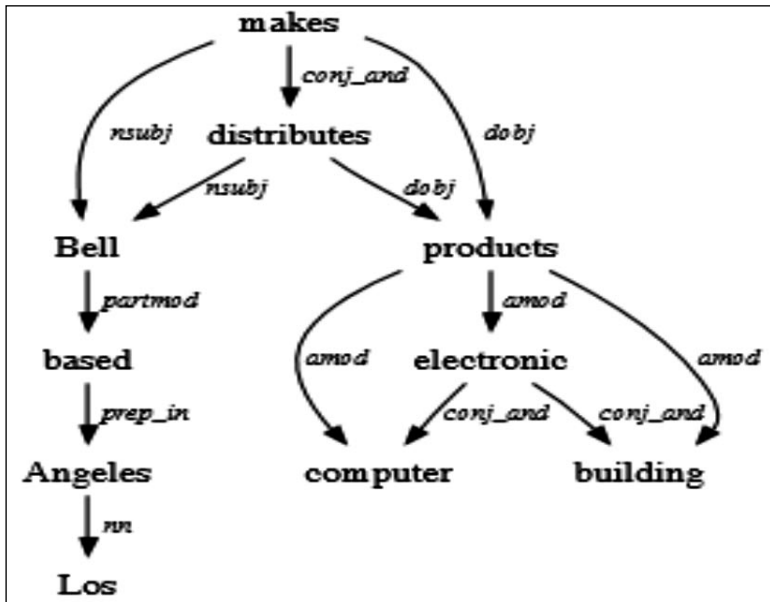
2. irudia. Bell, based in Los Angeles, makes and distributes electronic, computer and building products esaldiaren irudikapen grafikoa SDak baliatuta [5].
