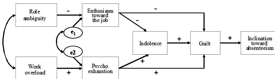
Figure 1. Hypothesized model.
